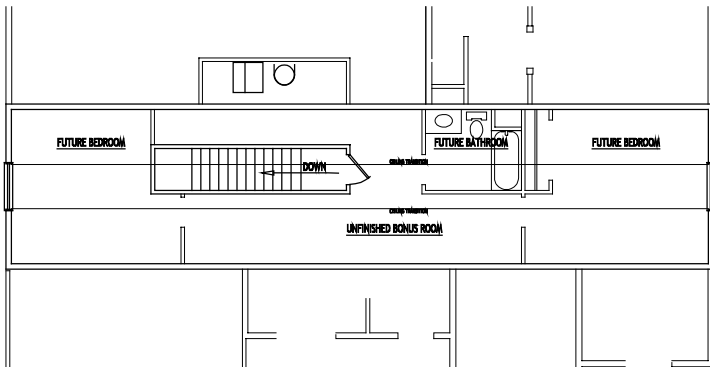
UPPER FLOOR LAYOUT
