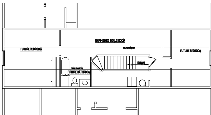
UPPER FLOOR LAYOUT
