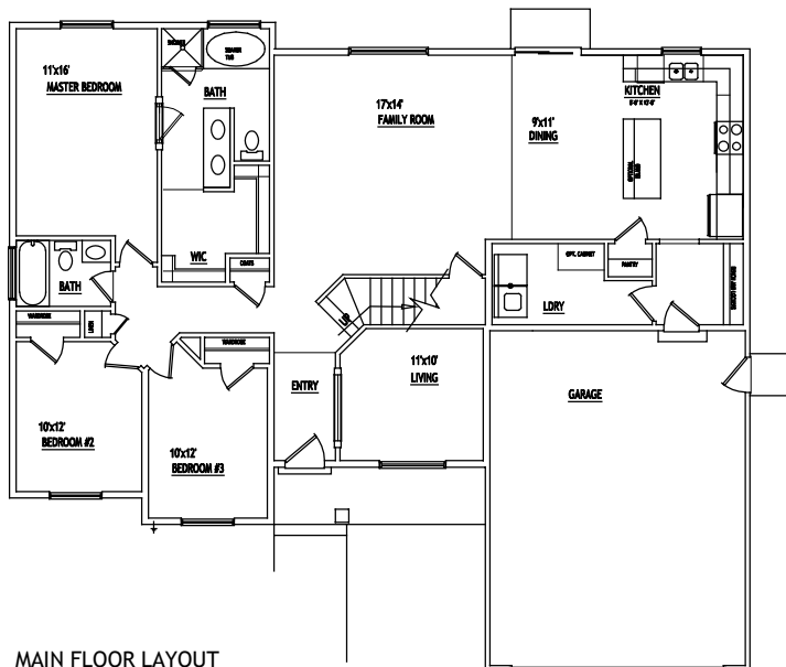
MAIN FLOOR LAYOUT
