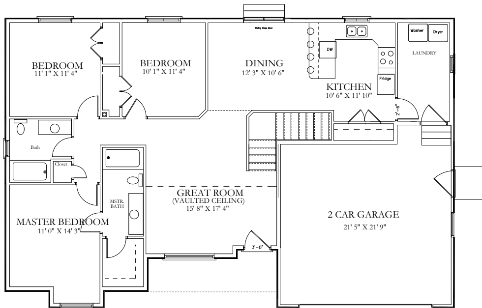
1 Main Floor Plan 21.1 Scale: NTS
