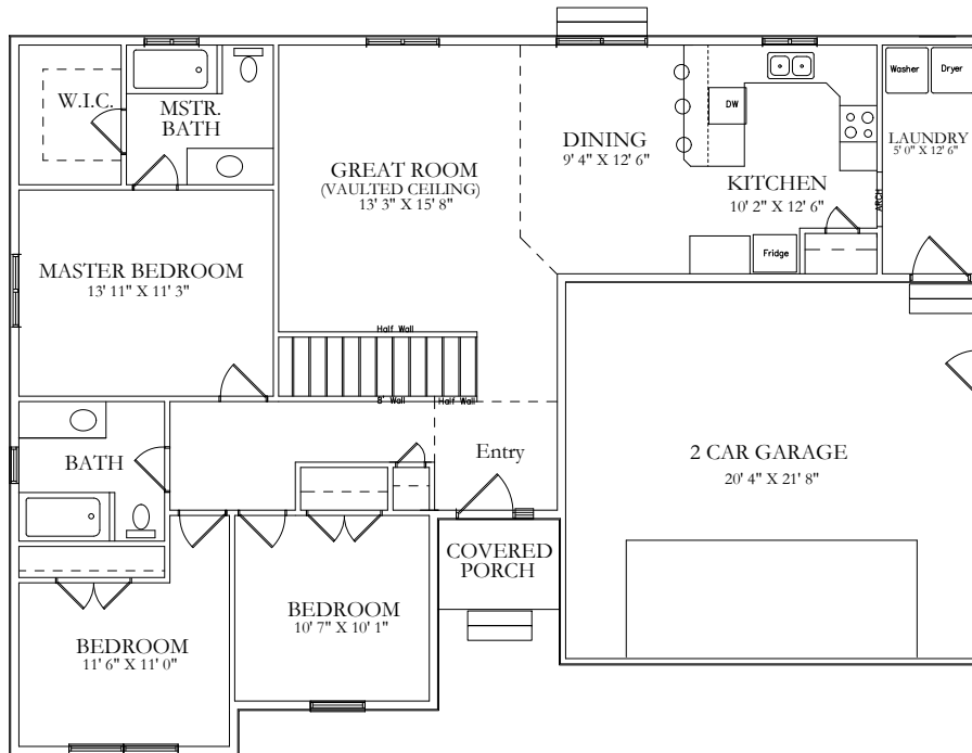
1 Main Floor Plan Scale: NTS
