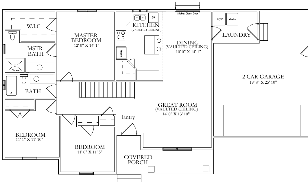
1 Main Floor Plan 21.1 Scale: NTS
