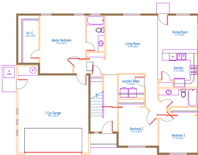
1 Main Floor Plan Scale: NTS
