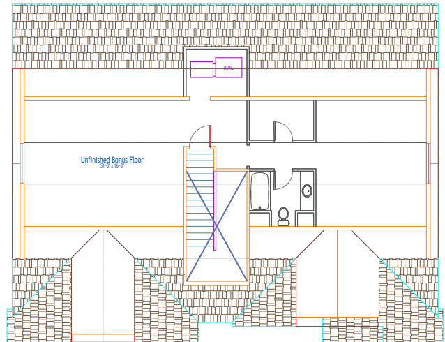
1 Bonus Floor Plan Scale: NTS
