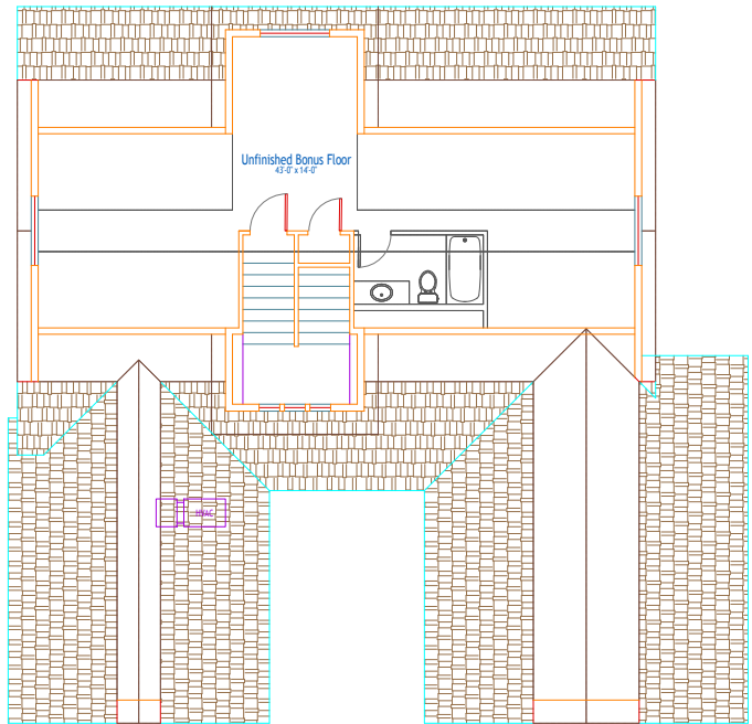
1 Bonus Floor Plan Scale: NTS
