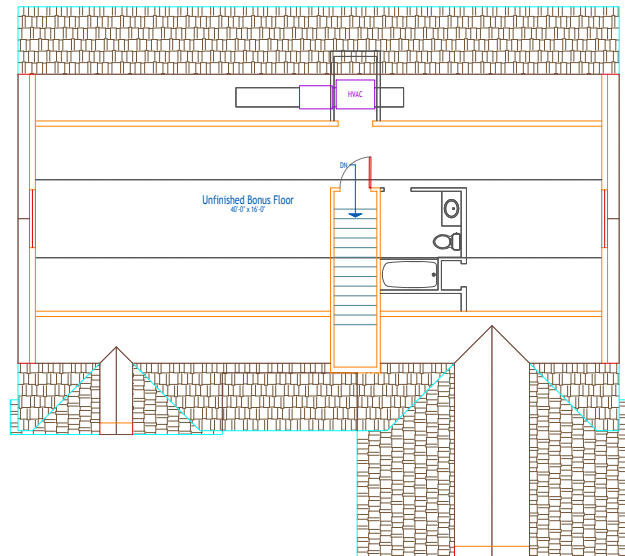
1 Bonus Floor Plan Scale: NTS
