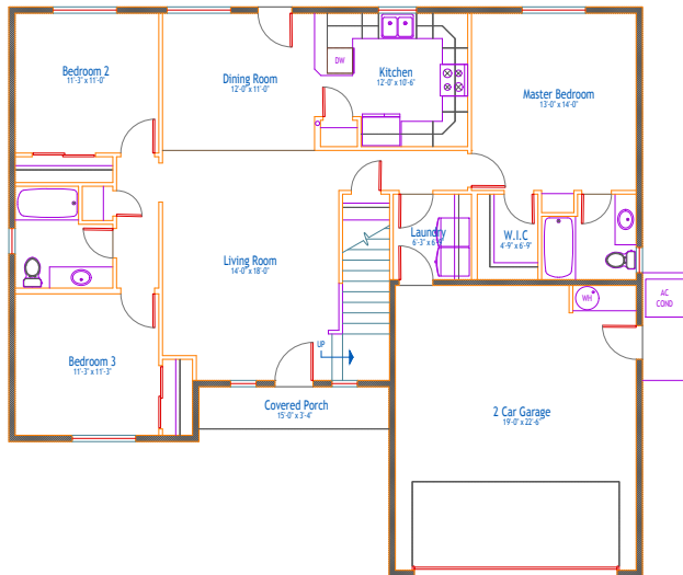
1 Main Floor Plan Scale: NTS
