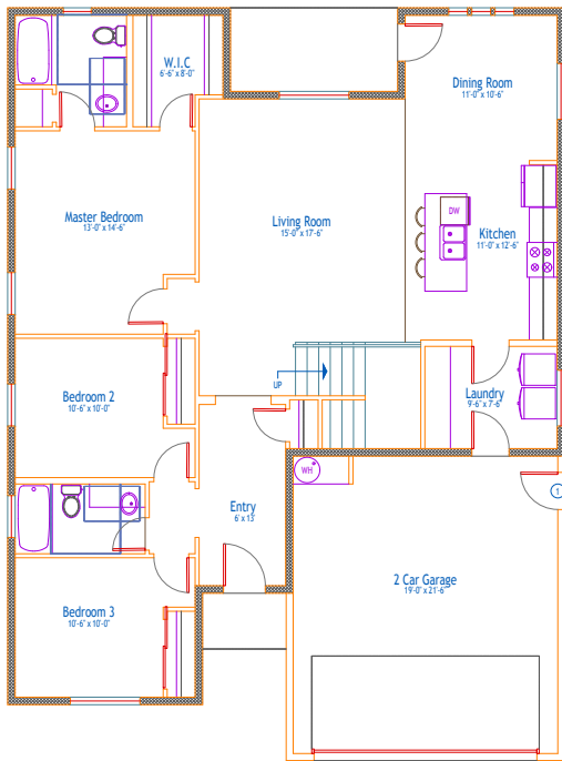
1 Main Floor Plan Scale: NTS
