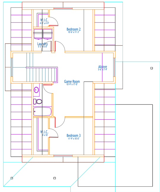
1 Bonus Floor Plan Scale: NTS
