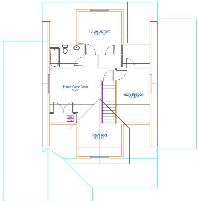
1 Bonus Floor Plan Z1.2 Scale: NTS
