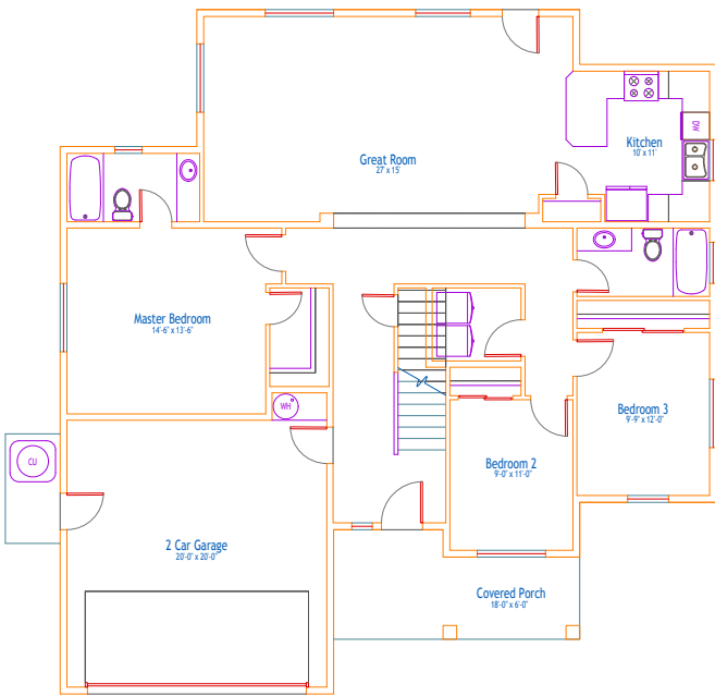
1 Main Floor Plan Z1.1 Scale: NTS
