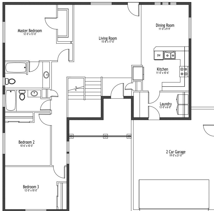
1 Main Floor Plan 21.1 Scale: NTS
