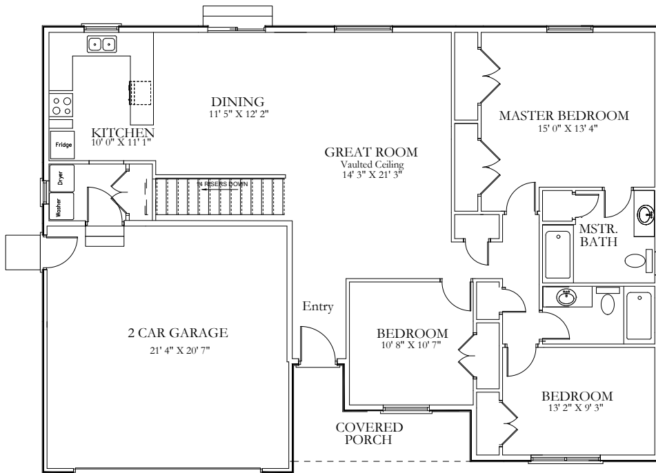
1 Main Floor Plan 21:1 Scale: NTS
